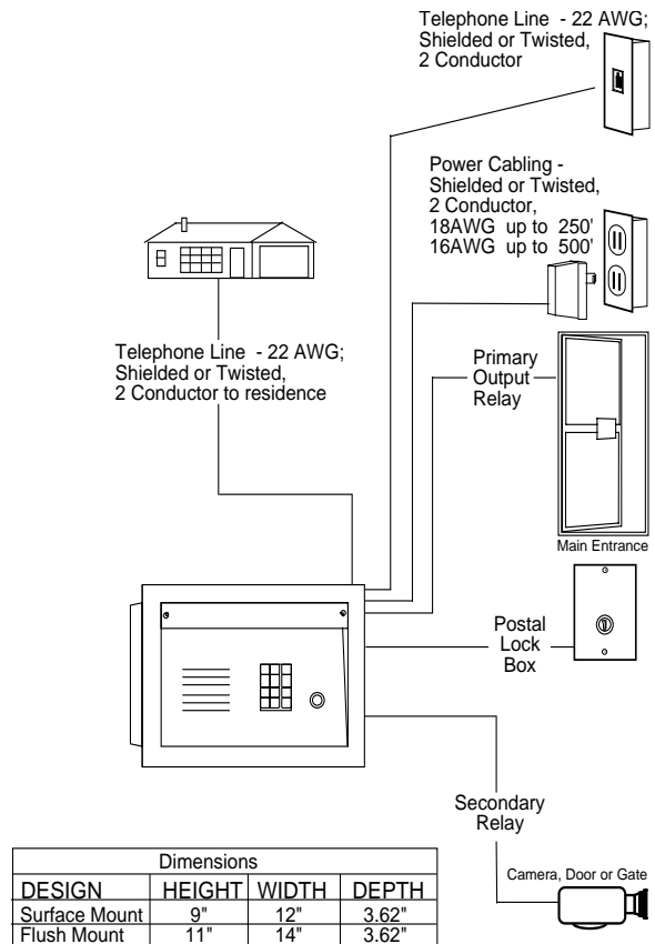
Hookup Specifications
